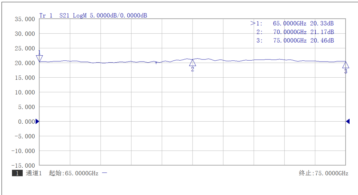
Gain vs Frequency 65-75GHz
