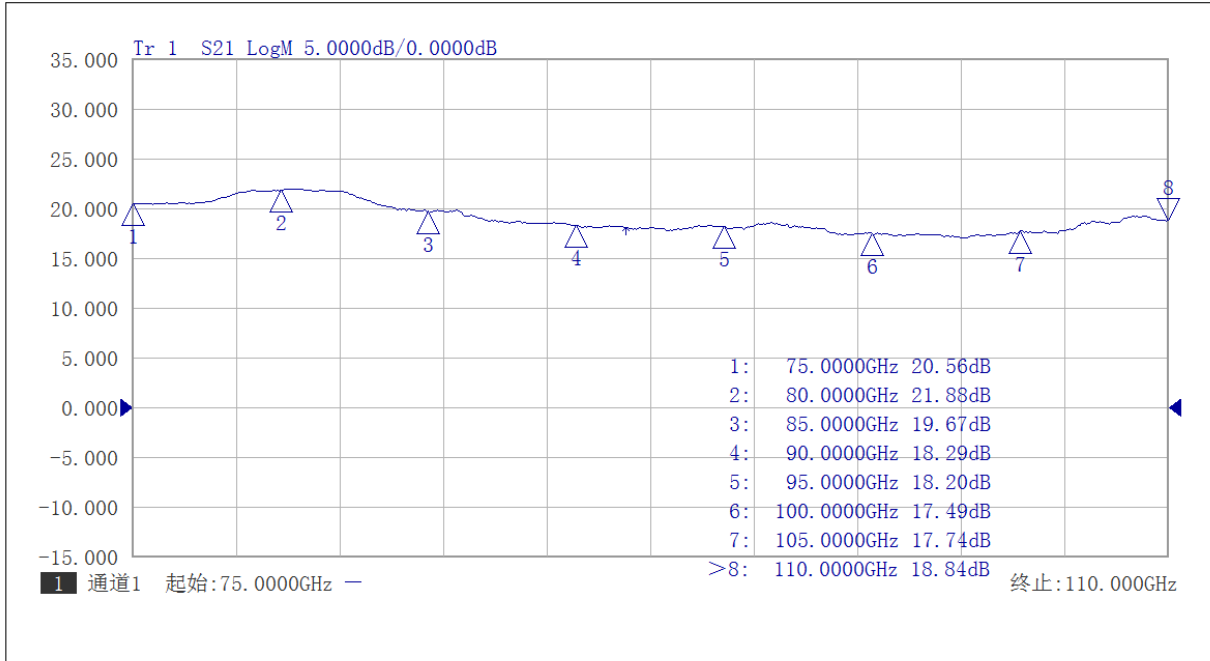
Gain vs Frequency 75-115GHz
